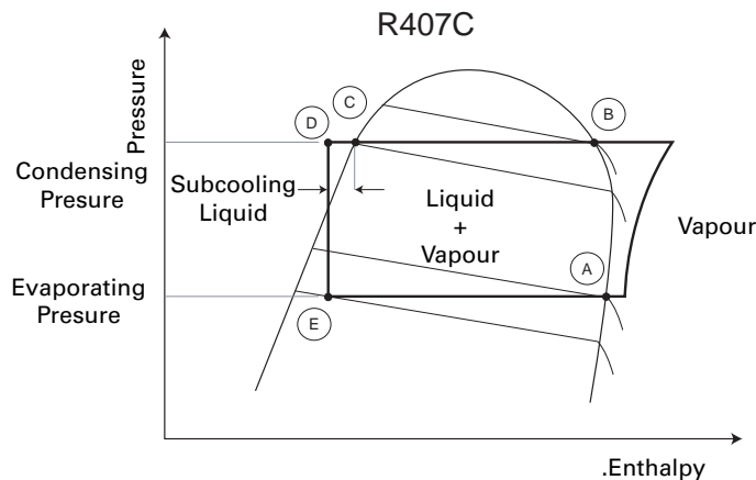
Figure 3 - R407C Refrigerant cycle
